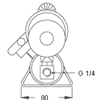
Front end view
